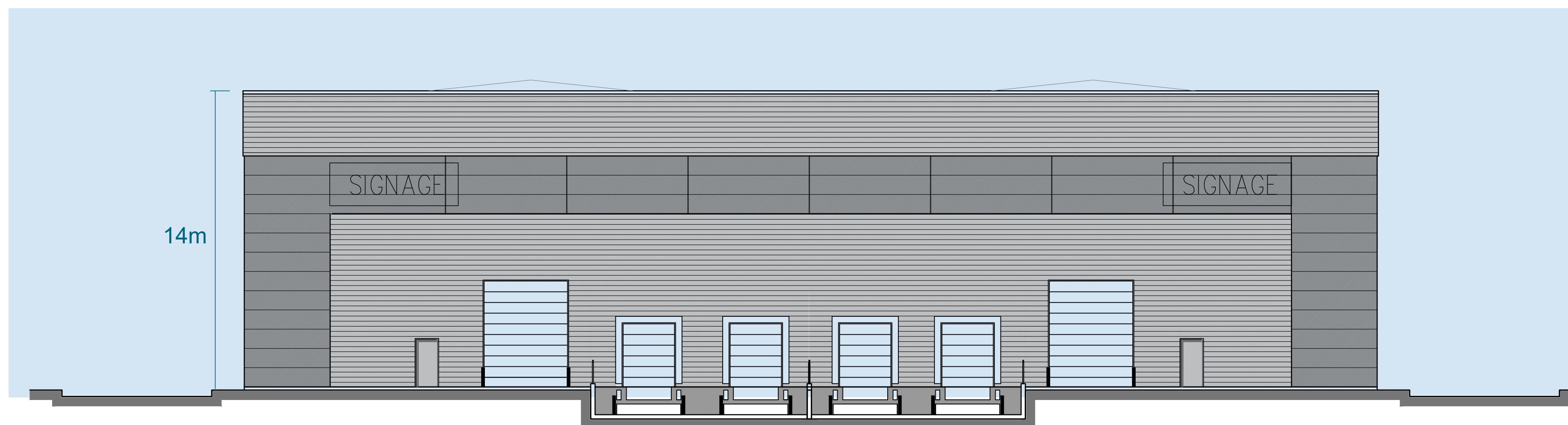
North Elevation
